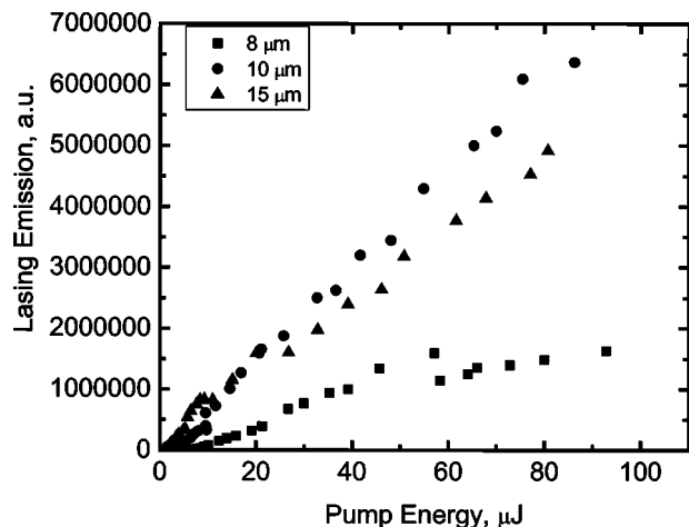
FIGURE 6 Cell gap effect on the lasing emission.
